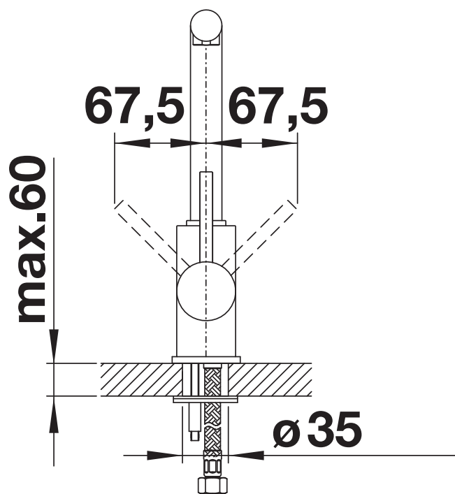
Side view lever
